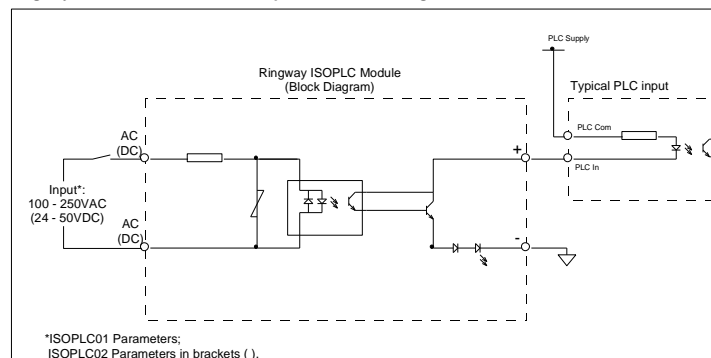
Ringway ISOPLC Module wired in Open Collector Configuration
